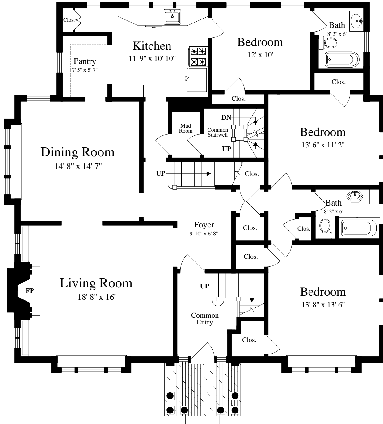
FIRST FLOOR (ceiling = 8' 4")
