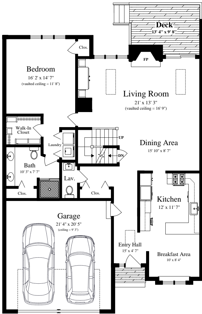
FIRST FLOOR (ceiling = 8')
