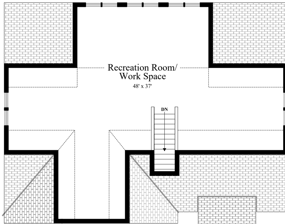
THIRD FLOOR (ceiling = 7')
