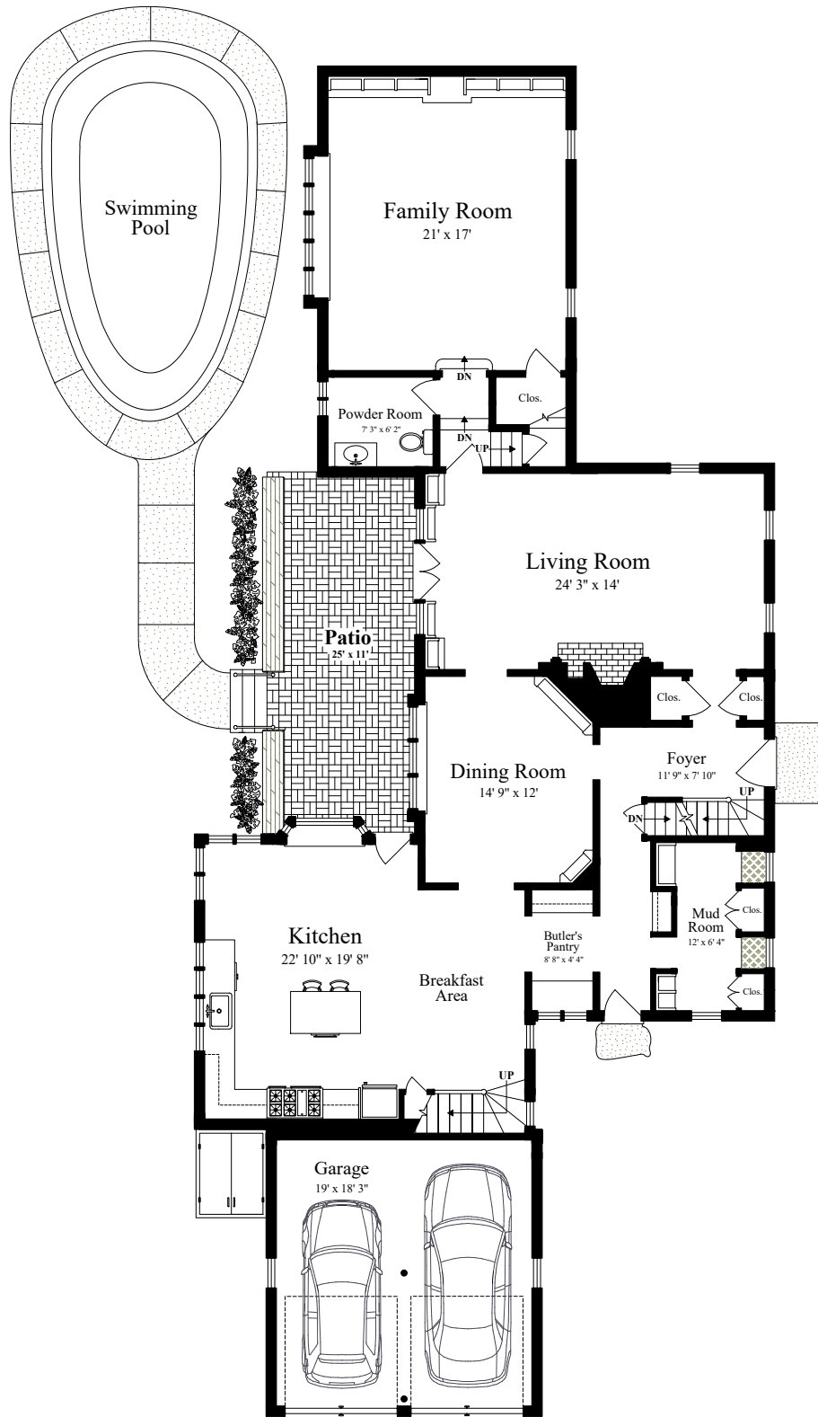
FIRST FLOOR (ceiling = 7' 8")
