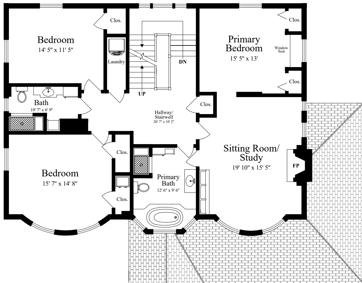
SECOND FLOOR (ceiling = 9')
