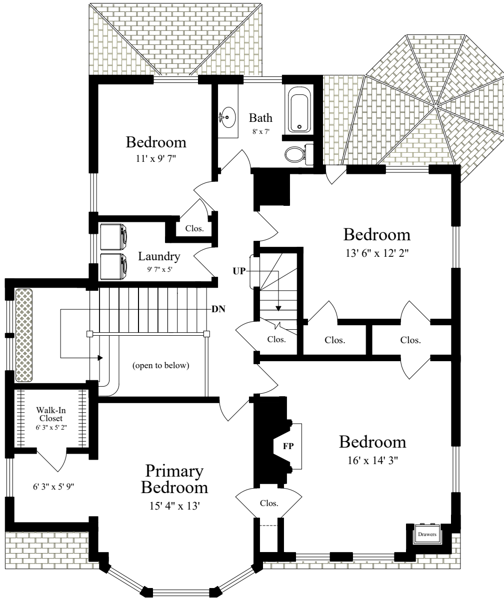
SECOND FLOOR (ceiling = 8' 7")
