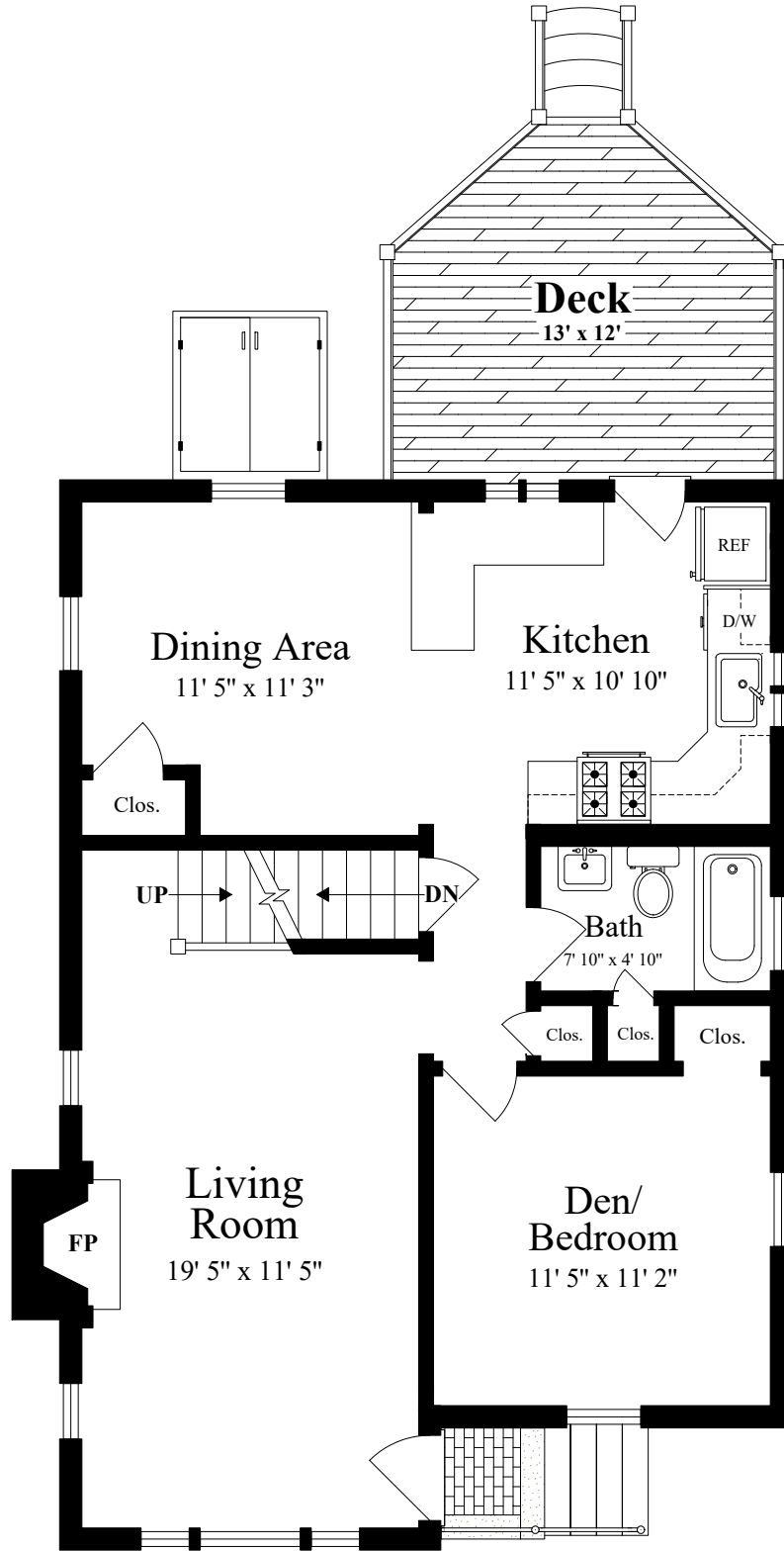
FIRST FLOOR (ceiling = 7' 5")
