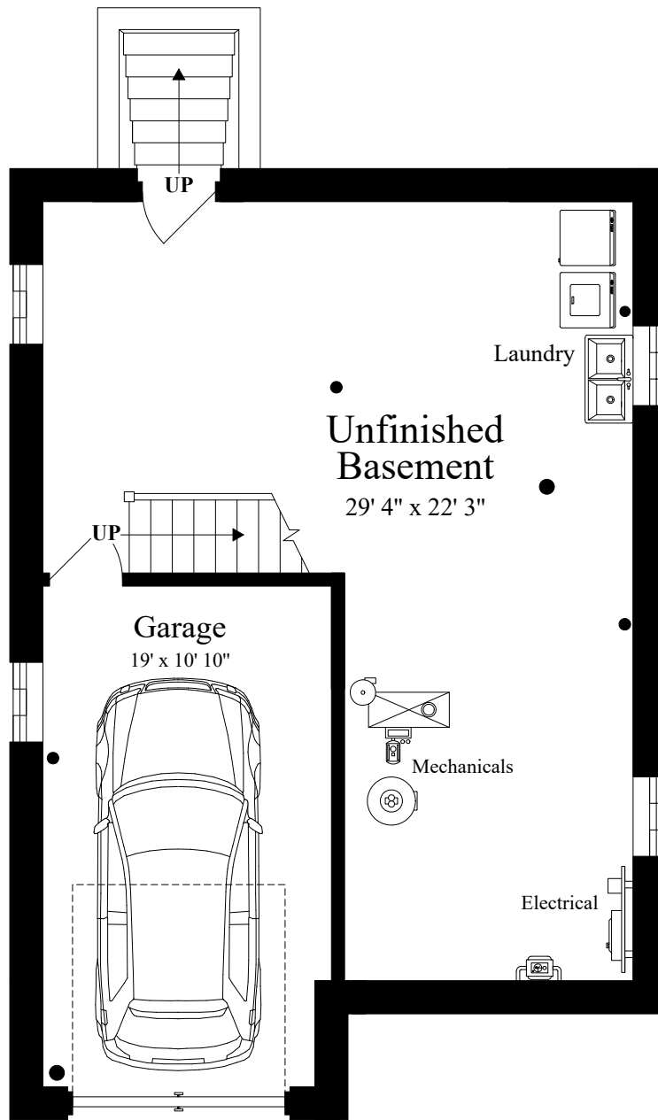
LOWER LEVEL (ceiling = 7' 1')
