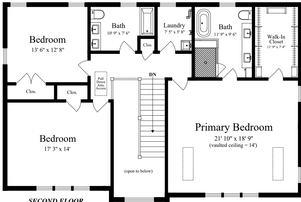
SECOND FLOOR (ceiling = 9')
