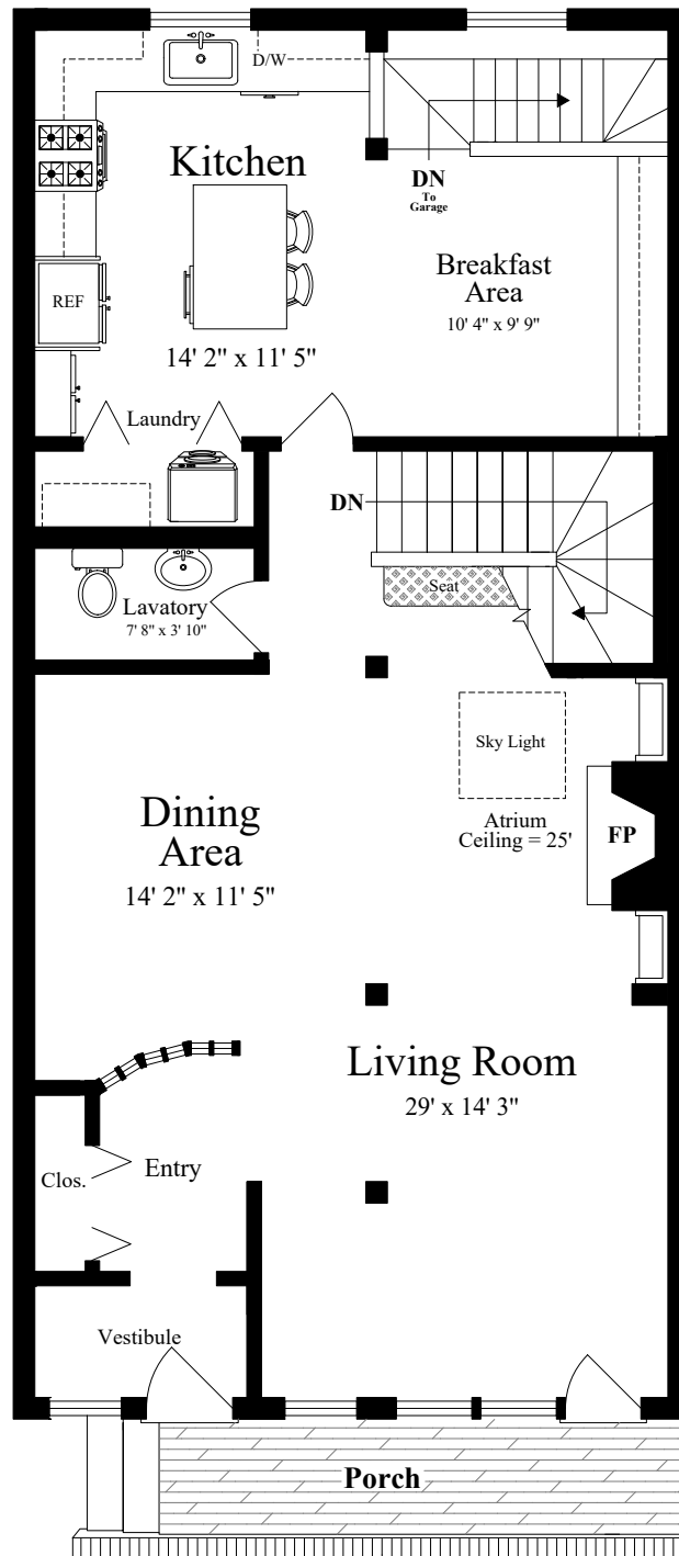
FIRST FLOOR (ceiling = 8' 3")
