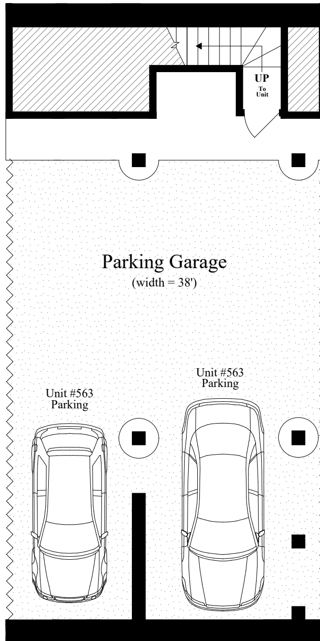
LOWER LEVEL (ceiling = 7' 2")
