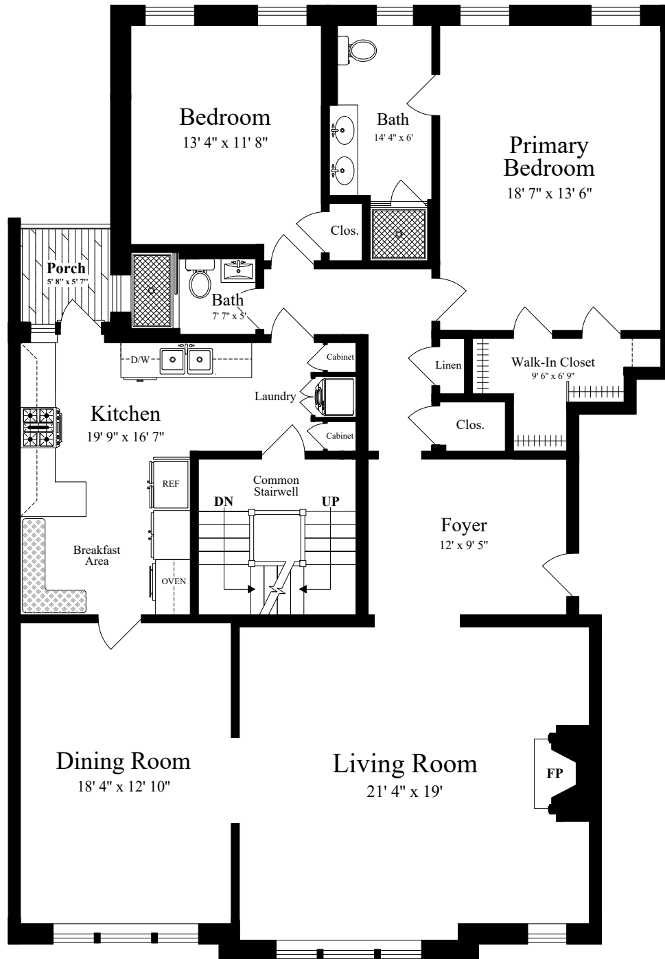
FIRST FLOOR (ceiling = 9')
