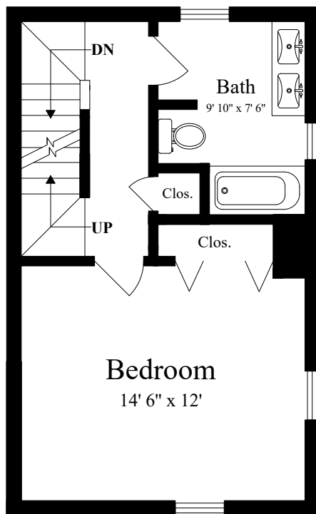
SECOND FLOOR (ceiling = 8')
