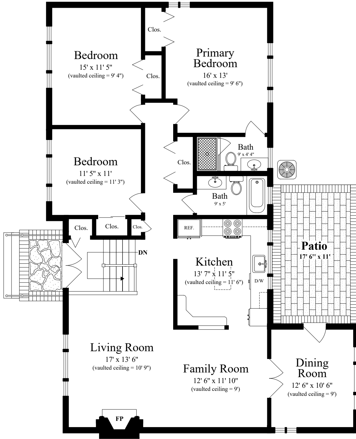
FIRST FLOOR (vaulted ceiling = 11' 6")
