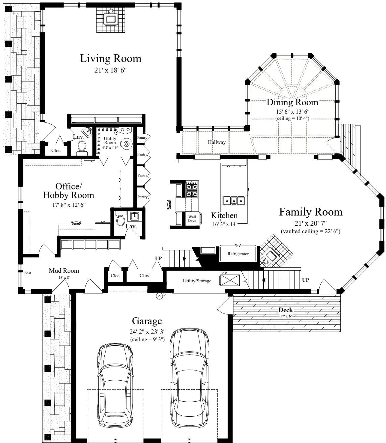
FIRST FLOOR (ceiling = 8' 6")
