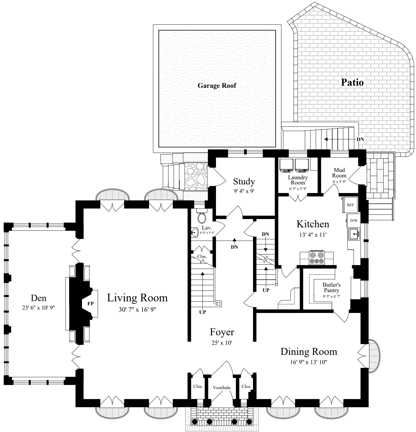
FIRST FLOOR (ceiling = 8' 6")
