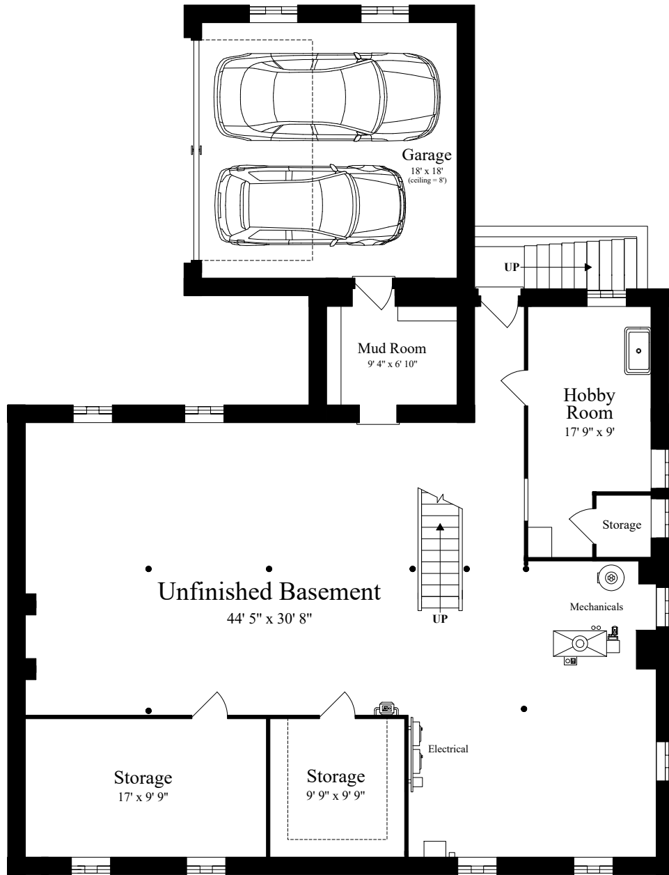
LOWER LEVEL (ceiling = 7' 5")
