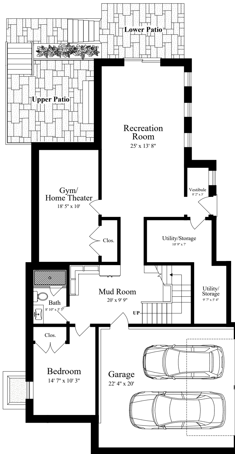
LOWER LEVEL
