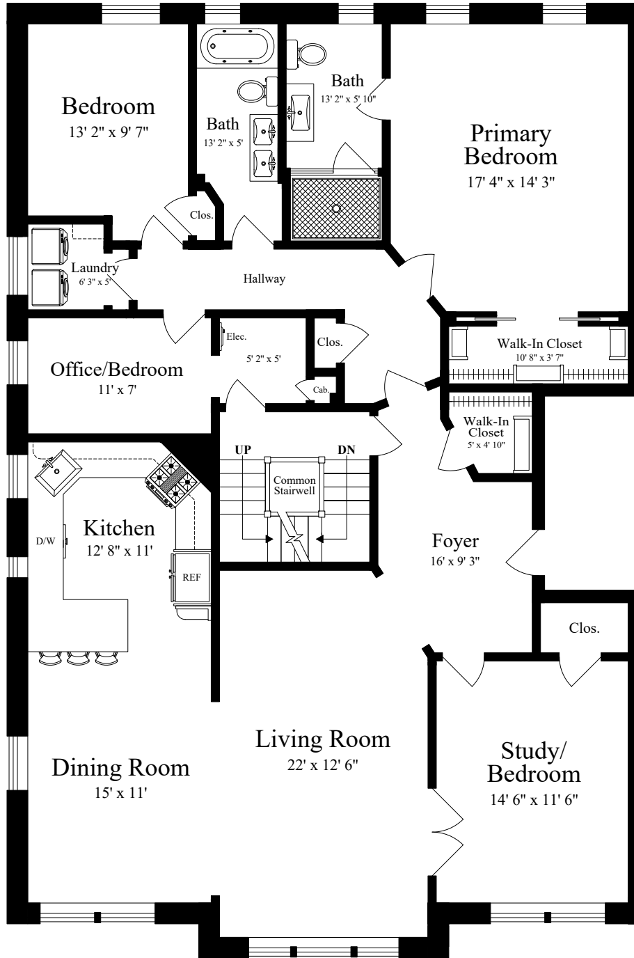
THIRD FLOOR (ceiling = 8' 8")
