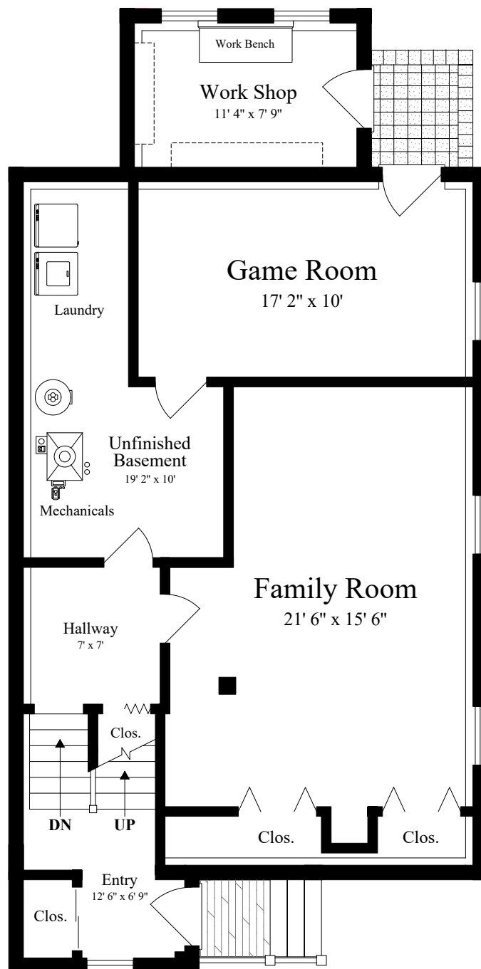
LOWER LEVEL (ceiling = 7')
