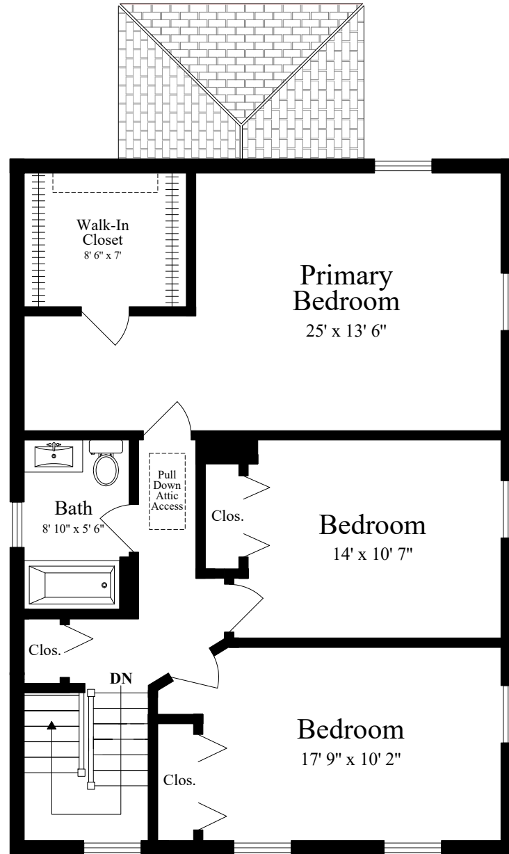
SECOND FLOOR (ceiling = 7' 6")
