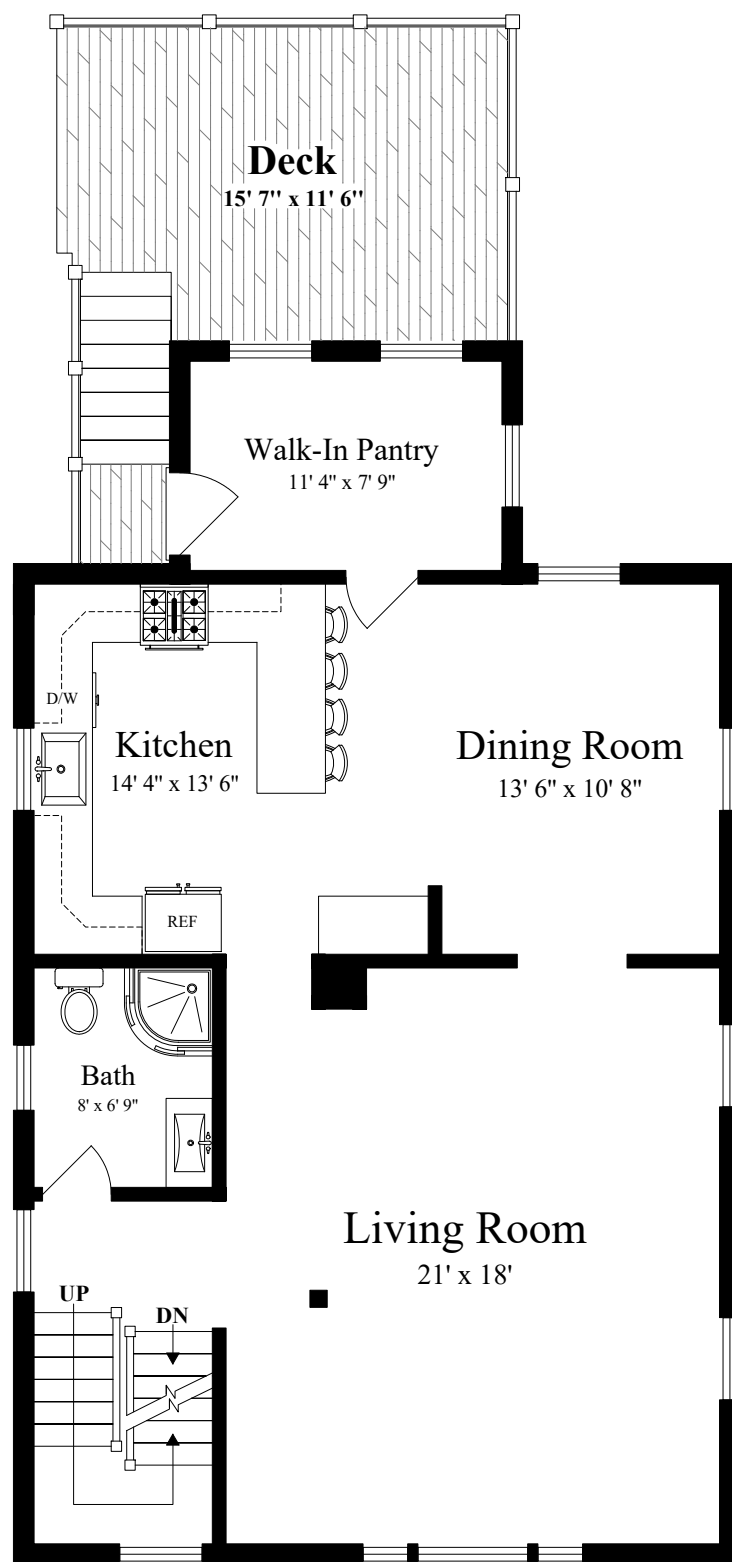
FIRST FLOOR (ceiling = 7' 6")
