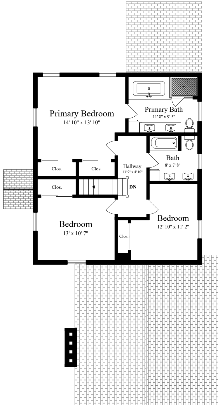
SECOND FLOOR
