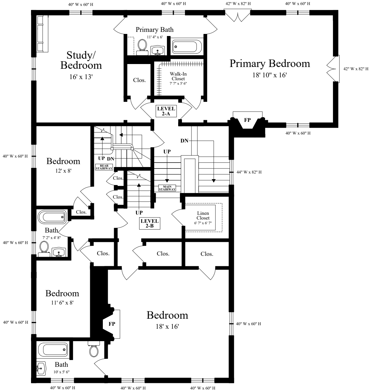
SECOND LEVELS (ceiling = 8')
