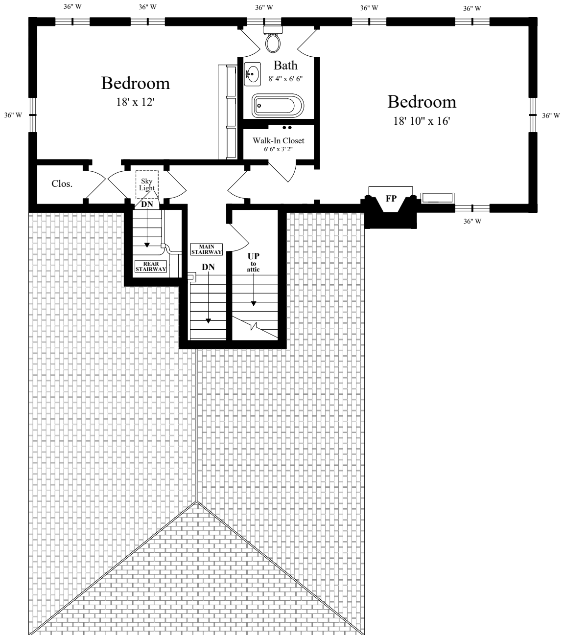
THIRD LEVEL (ceiling = 8')
