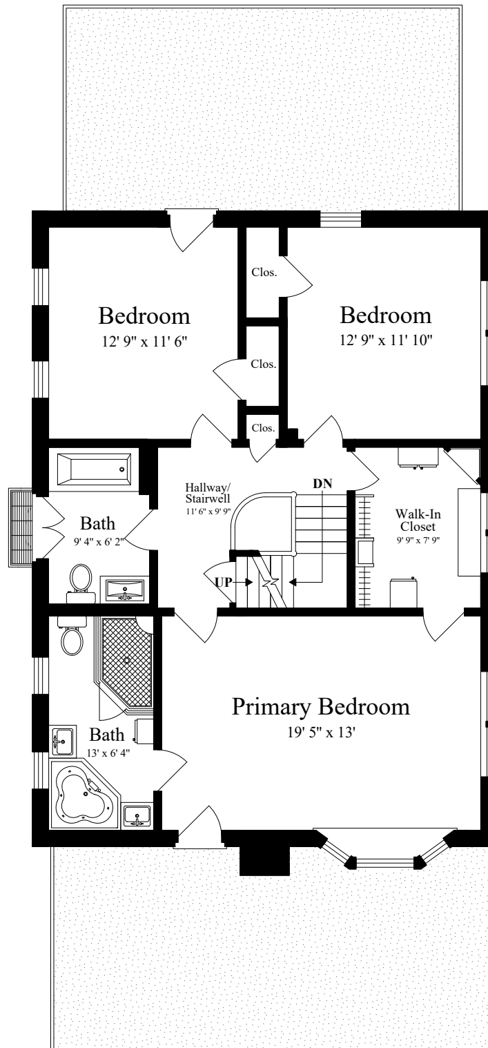
SECOND FLOOR (ceiling = 8')
