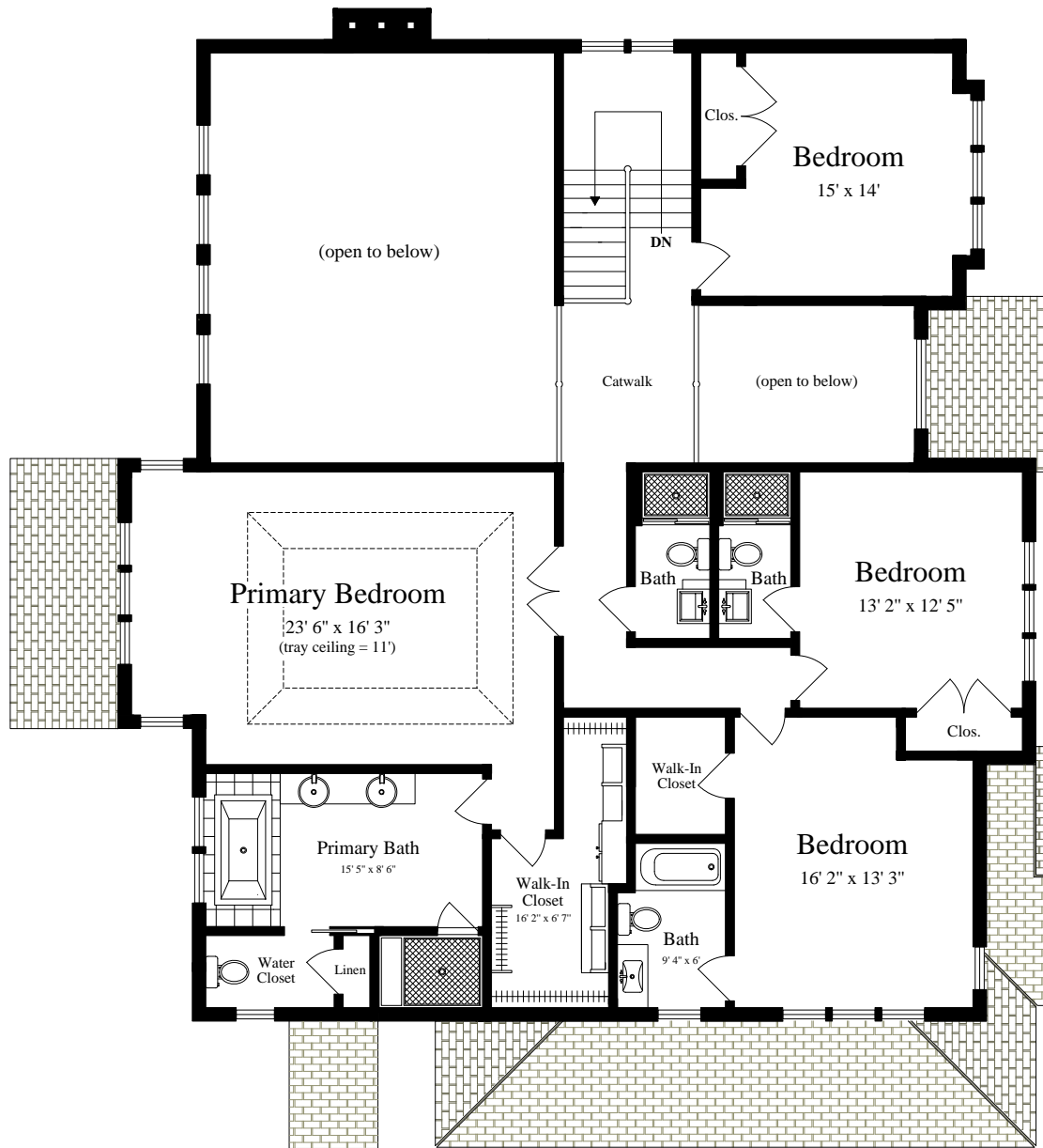
SECOND FLOOR (ceiling = 9')
