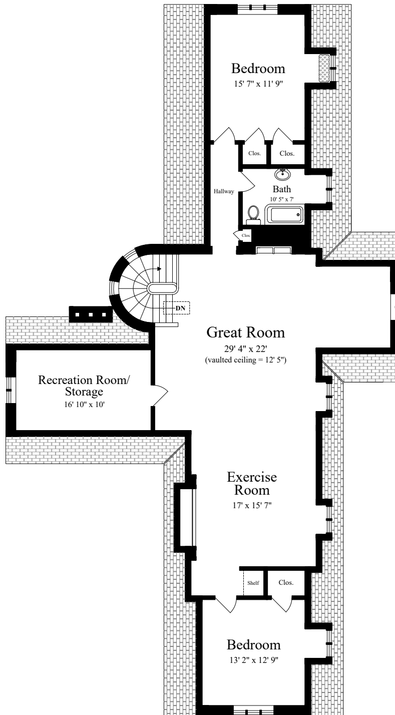
THIRD FLOOR (ceiling = 9' 6")
