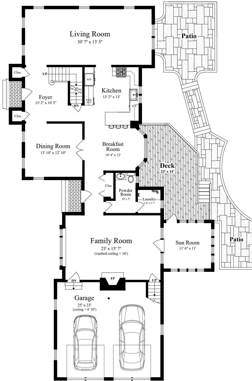
FIRST FLOOR (ceiling = 8' 6")
