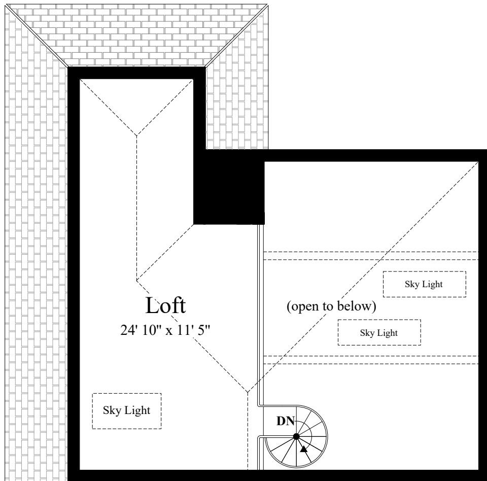
THIRD FLOOR (vaulted ceiling = 11' 6")
