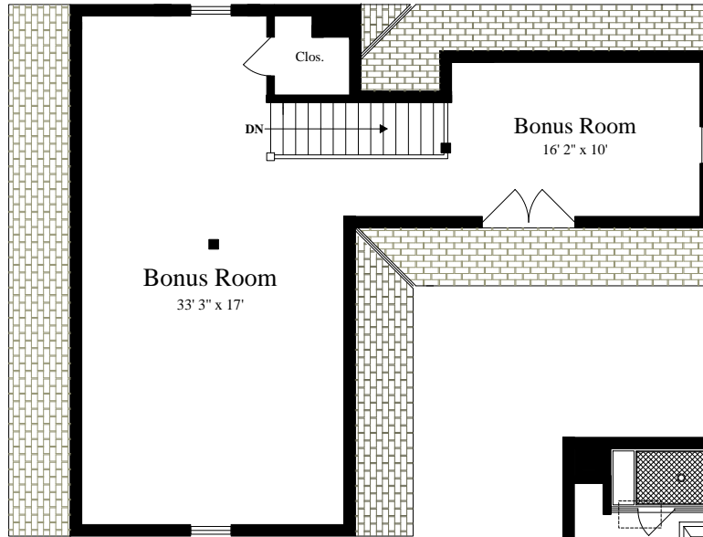
THIRD FLOOR (ceiling = 7')
