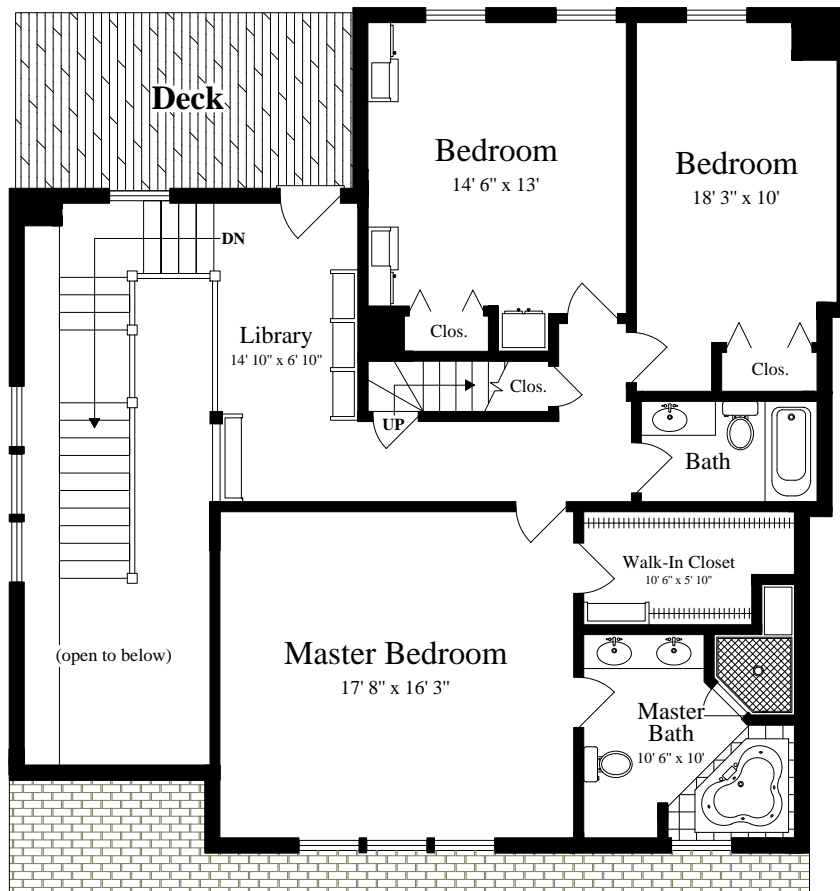
SECOND FLOOR (ceiling = 9')
