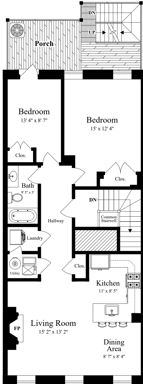
THIRD FLOOR (ceiling = 8' 6")
