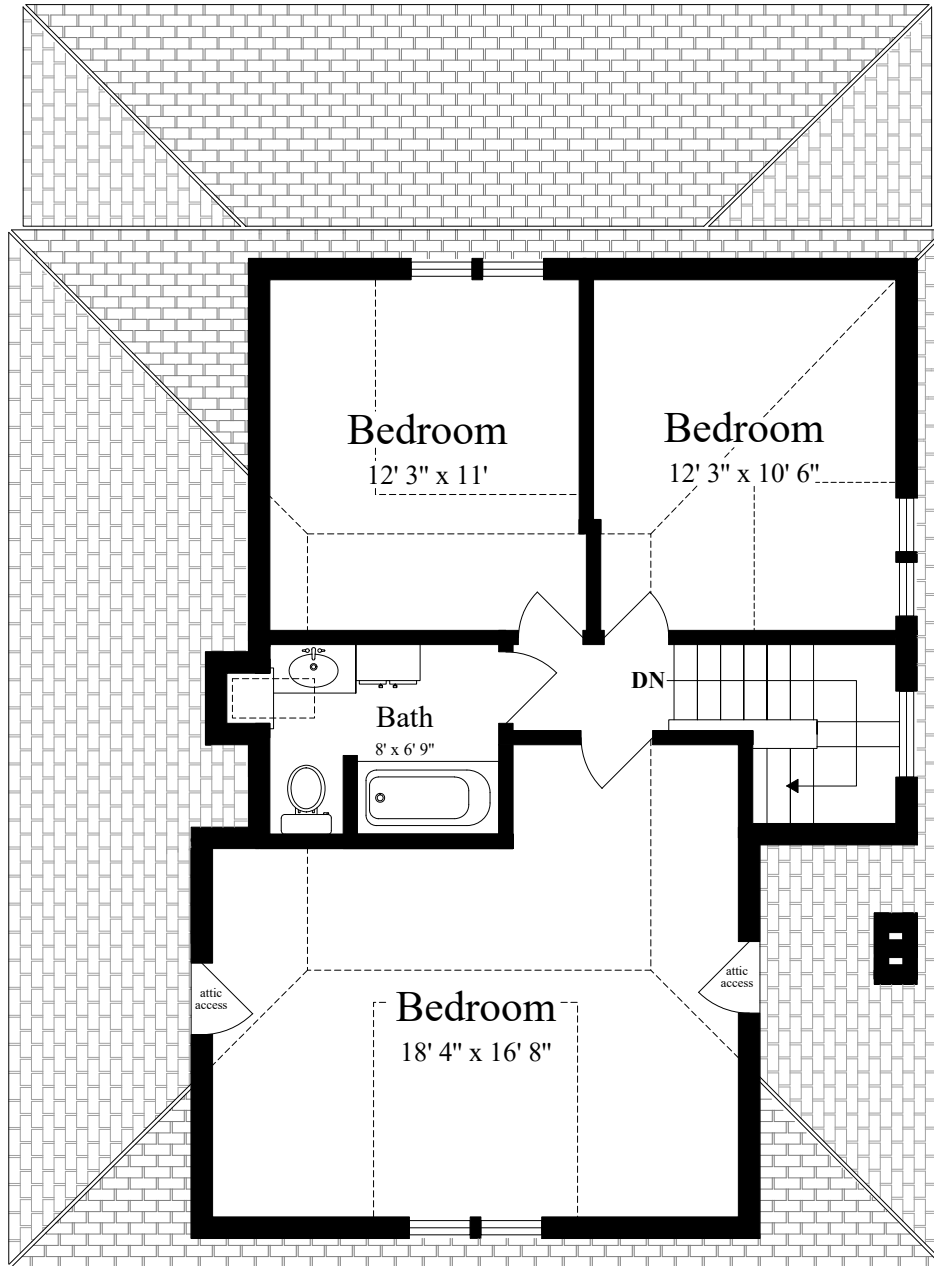
THIRD FLOOR (ceiling = 8')
