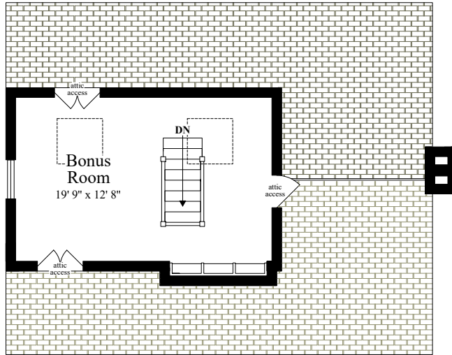
THIRD FLOOR (vaulted ceiling = 8')
