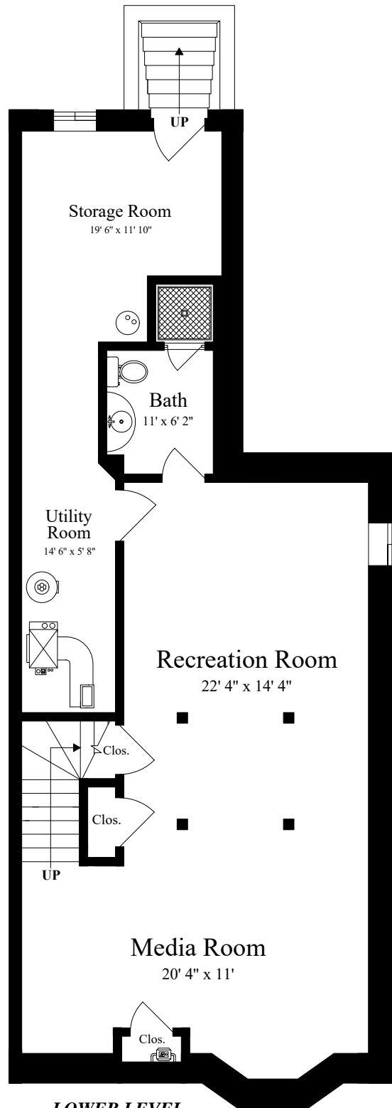
LOWER LEVEL (ceiling = 7' 7")
