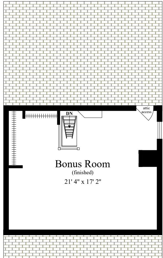
THIRD FLOOR (ceiling = 9')
