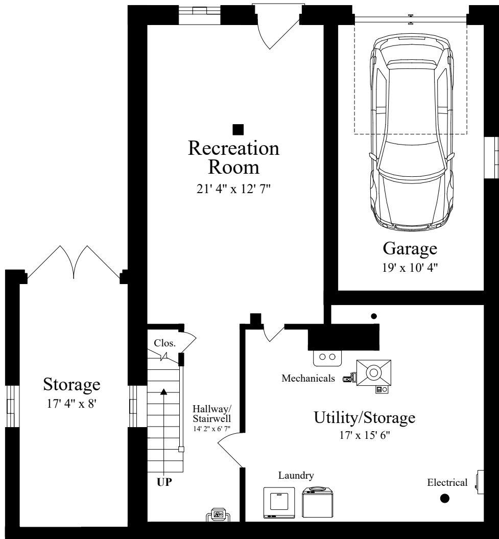
LOWER LEVEL (ceiling = 7' 3")
