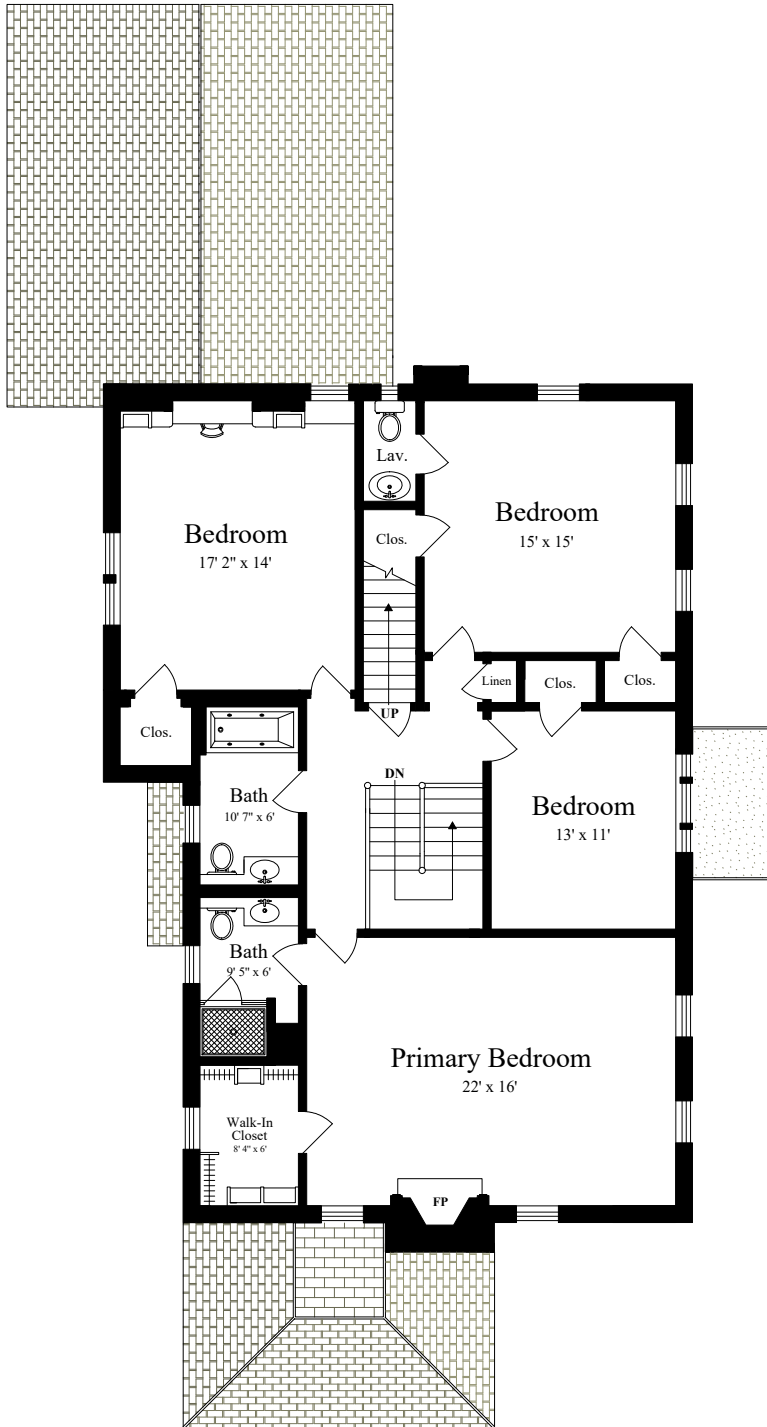
SECOND FLOOR (ceiling = 8' 3")
