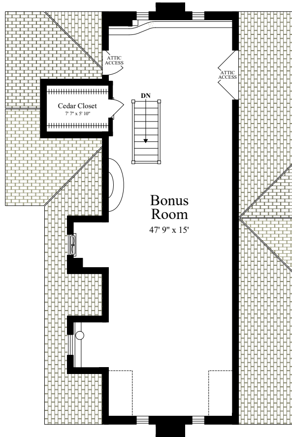
THIRD FLOOR (ceiling = 7' 1")
